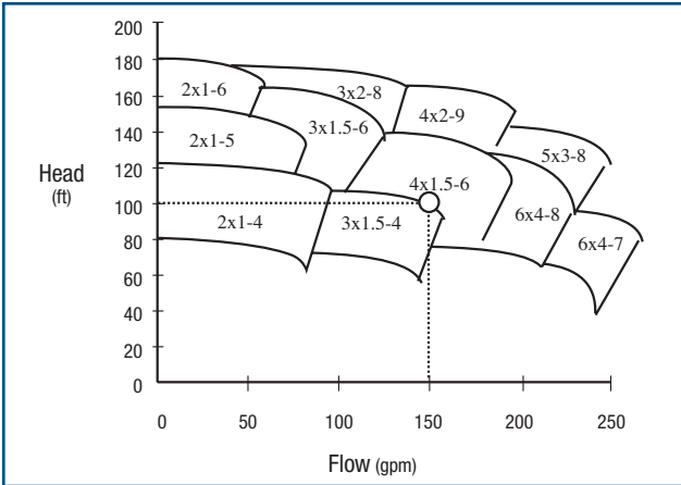
Figure 11. Family of Pump Performance Curves
